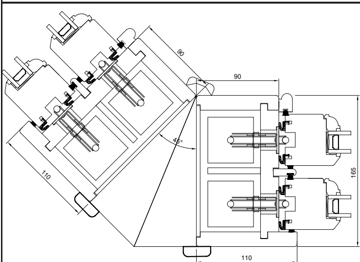
Option for Section C-C 45° corner post
