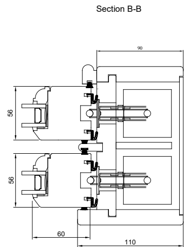
Option of inside and outside groove
