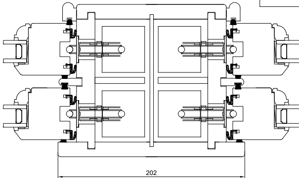
Section B-B SOLID MULLION OPTION
