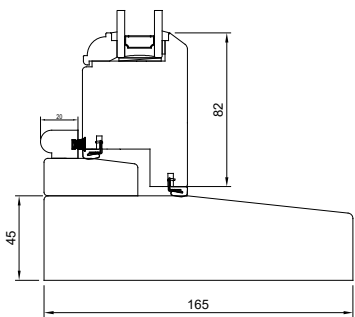
Section B-B SOLID MULLION OPTION
